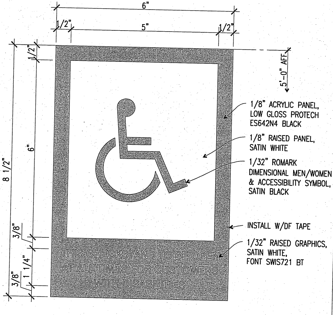
C1 ACCESSIBLE CASHWRAP SIGN 6"=1'-0" SIGNAGE FOLD
