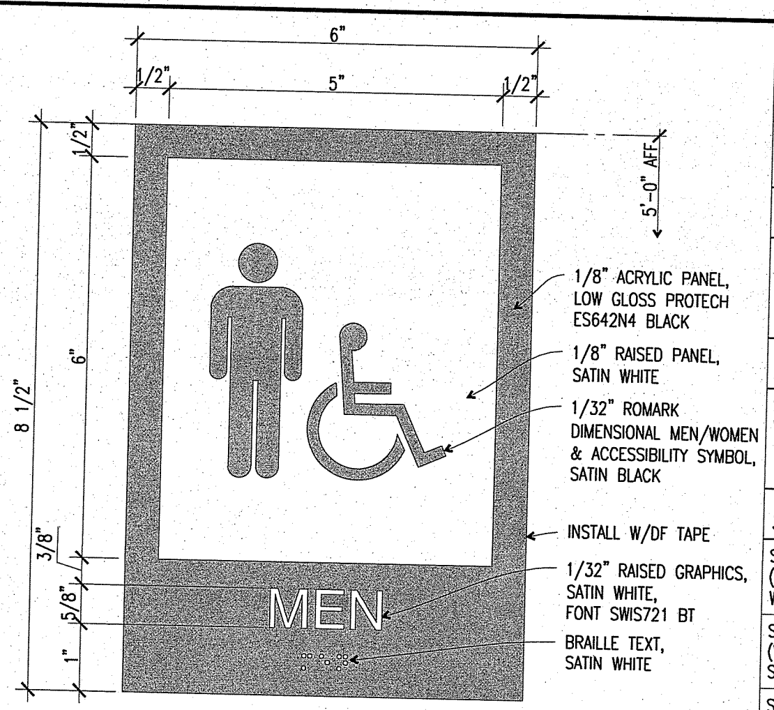
E7 PUBLIC RESTROOM SIGNAGE 6"=1'-0" SIGNAGE FOLD
