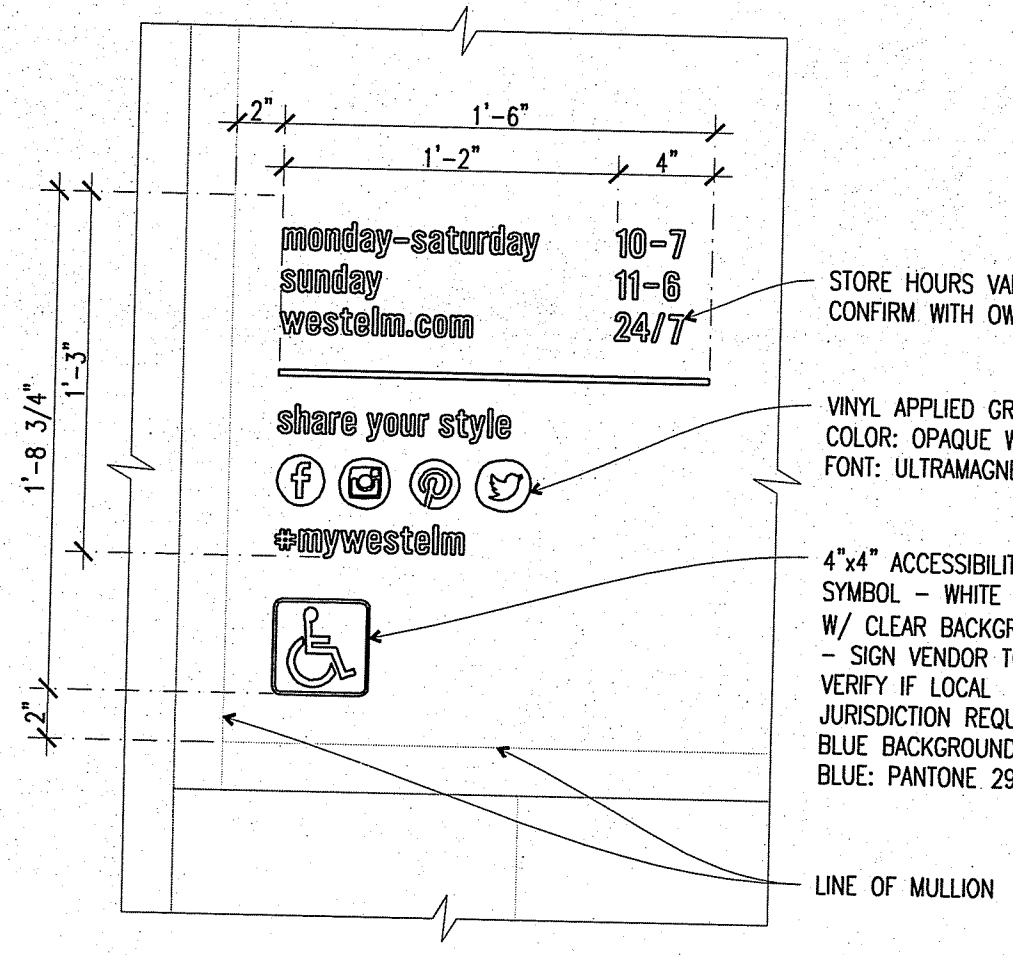
A1 STORE HOURS GRAPHICS - ACCESSIBLE 1 1/2"=1'-0" SIGNAGE FOLD
