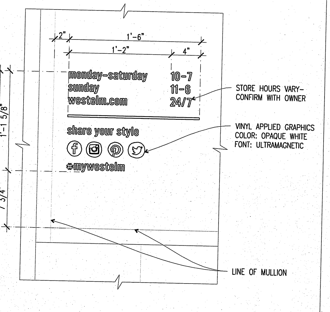
A1 STORE HOURS GRAPHICS 1 1/2"=1'-0" SIGNAGE FOLD
