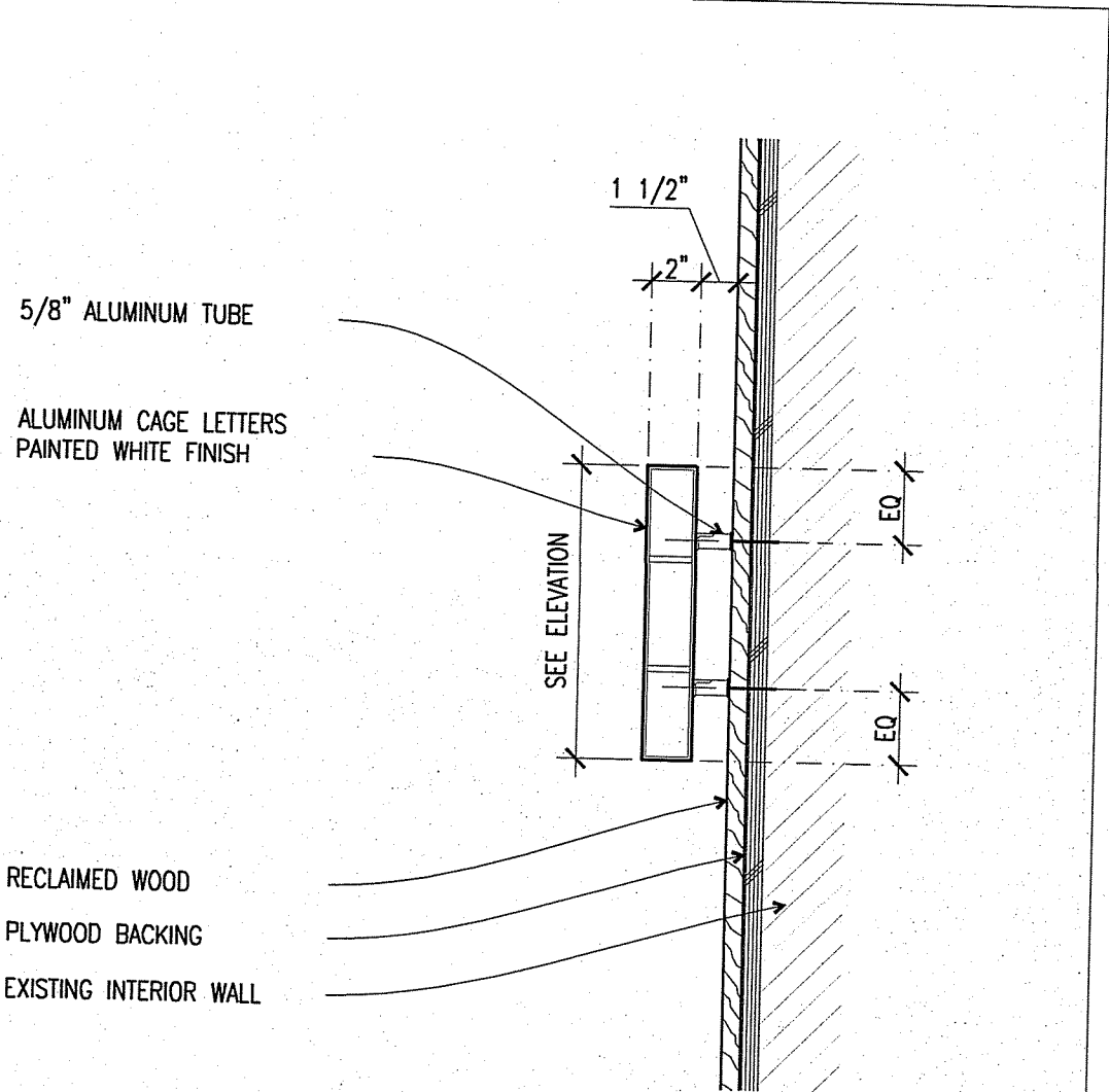
A5 WALL-MOUNTED CAGE SIGNAGE 1 1/2"=1'-0" SIGNAGE FOLD
