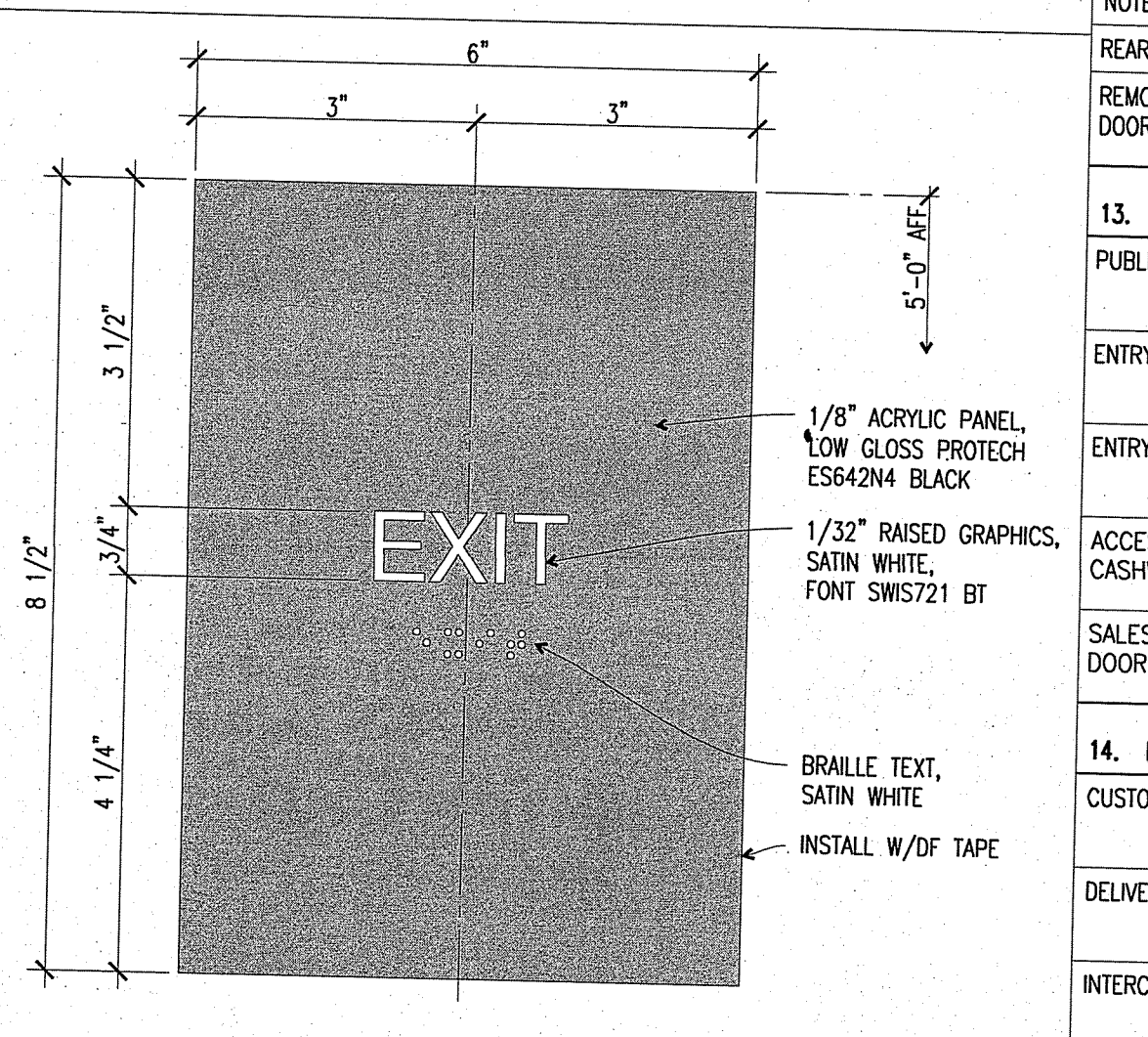
A7 TACTILE EXIT SIGNAGE 6"=1'-0" SIGNAGE FOLD
