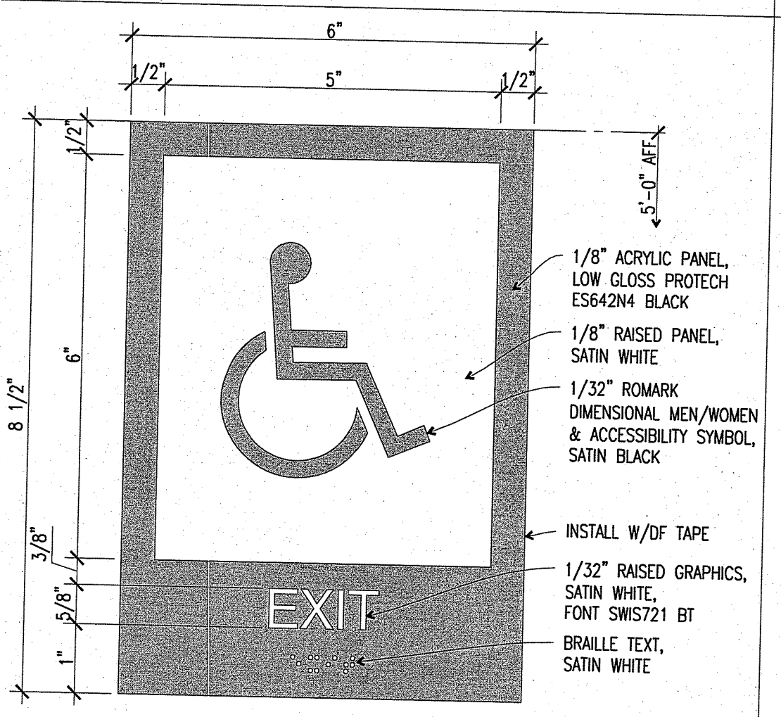
C3 ACCESSIBLE EXIT SIGNAGE 6"=1'-0" SIGNAGE FOLD
