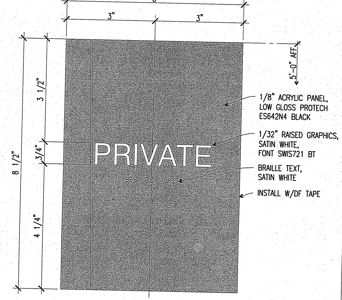
E3 PRIVATE SIGNAGE 6"=1'-0" SIGNAGE FOLD
