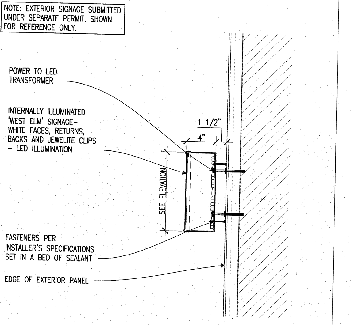
A3 WALL-MOUNTED SIGNAGE 1 1/2"=1'-0" SIGNAGE FOLD
