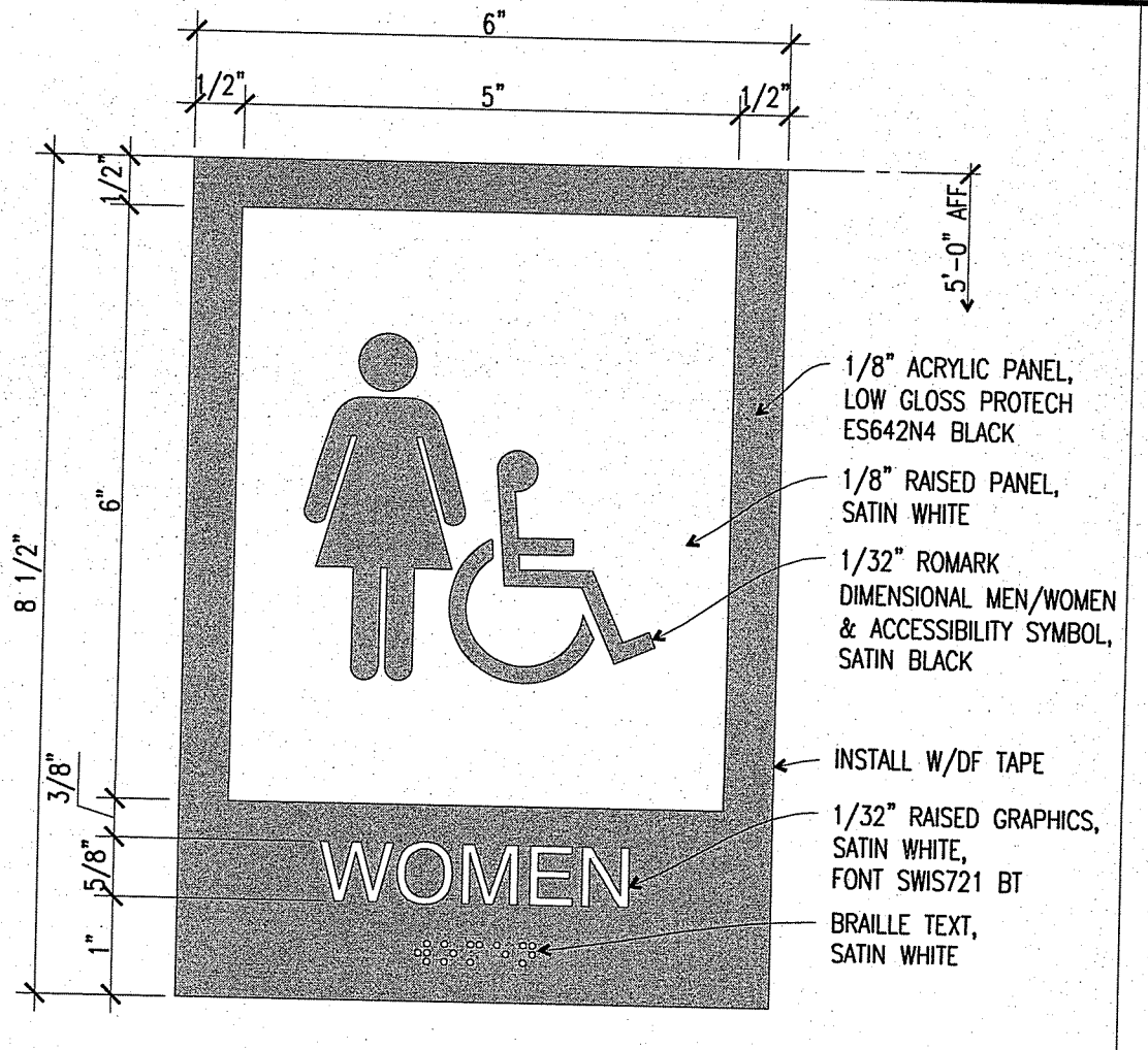
E5 PUBLIC RESTROOM SIGNAGE 6"=1'-0" SIGNAGE FOLD
